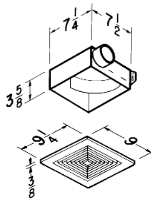
MODELS 676 & 684
