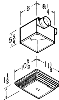
MODELS 676 & 684
