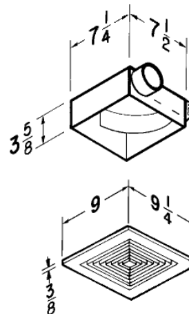
MODELS 688 & 689
