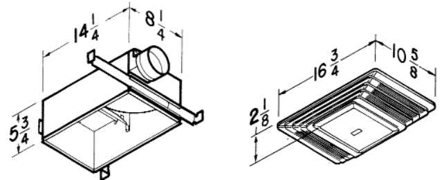
MODEL 696
