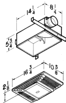
MODELS 655 & 657
