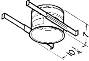
MODEL 504 HOUSING
