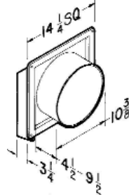
MODEL 508 HOUSING
