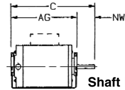
Shaft Dimensions
